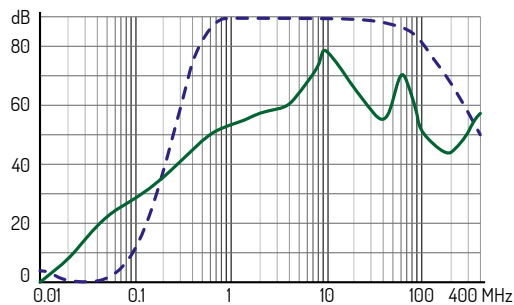
Filterkurve PX FILTER
